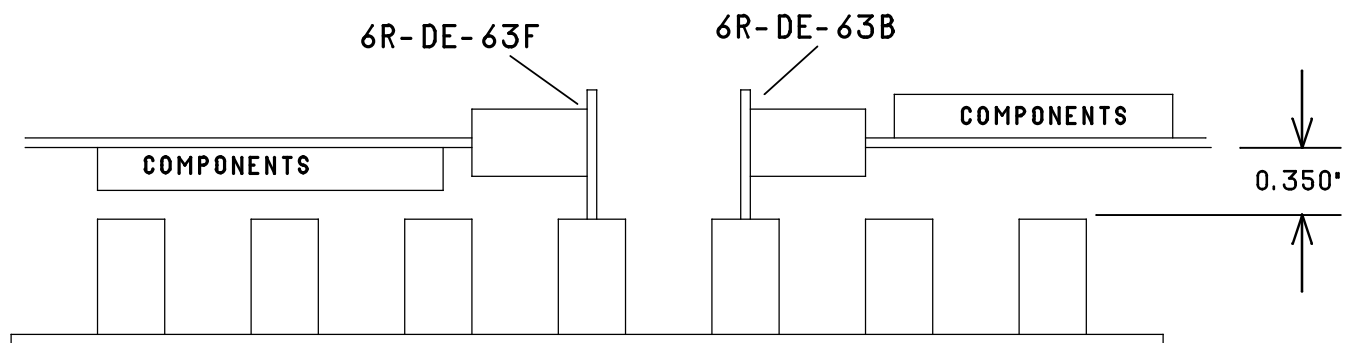
LOOKING FROM THE 'BRACKET' END OF THE ISA CARDS
